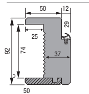
KM1 cloison 72 mm recouvrement
